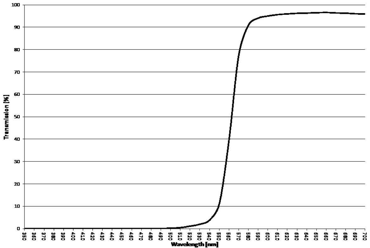
Spectral Transmittance
