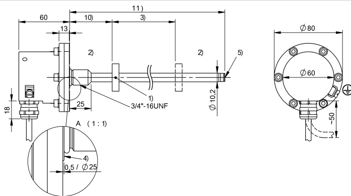
BTL5-Sxxxx-Mxxxx-Z-DEXB-Kxx
